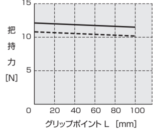
HP09FR-16-H
