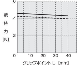
HP09FR-8-H
