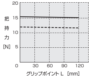
HP09FR-20-H
