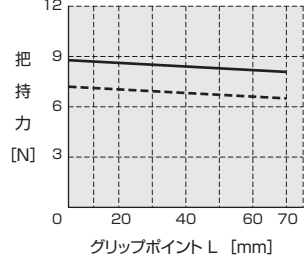
HP09FR-10-H
