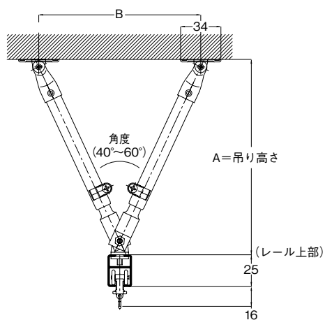
伸縮吊棒A
