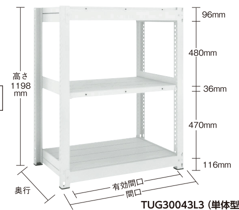
TUG30043L3 (単体型)
