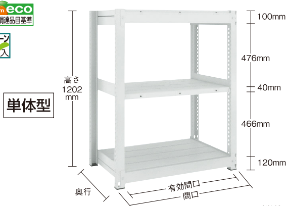
TUG45043L3 (単体型)
