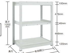
TUG60043L3 (単体型)
