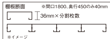
TUG3004SS
