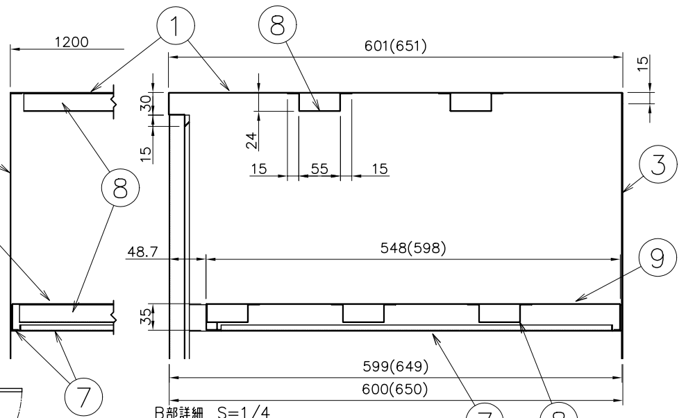
B部詳細 S=1/4
