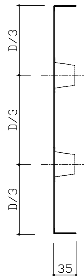
補強2本仕様
