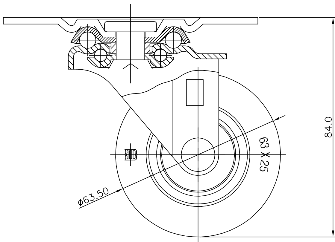
TP3625-01 CASTER
